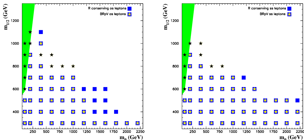
Figure 7: Same as figure 6 but for an integrated luminosity of 100 \text{ fb}^{-1} .
