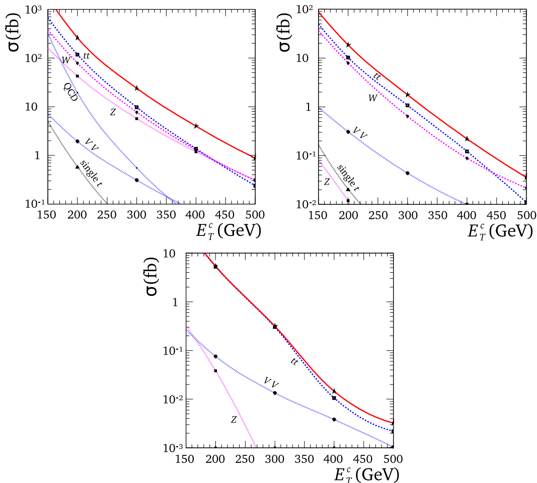
Figure 3: Composition of the inclusive (top left panel), one lepton (top right panel), opposite sign (lower panel) backgrounds. The top (red) solid lines stands for the total backgrounds while the blue dashed line corresponds to the t\bar{t} background, the magenta dashed lines corresponds to Wj , and the magenta dotted lines stands for the Zj process. The QCD background is represented by the dotted blue line while the dotted black lines stands for the single top production and VV is represented by the lower dotted blue line at small E_T^c .
