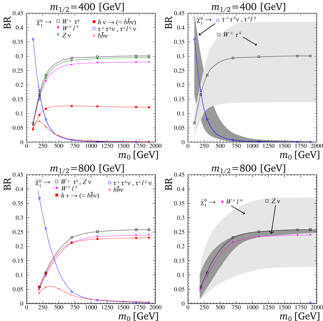
Figure 2: Lightest neutralino branching ratios as a function of m_0 for A_0 = -100 GeV, \tan\beta = 10 , and \mu > 0 . In the upper panels we have m_{1/2} = 400 GeV while the lower ones the correspond to m_{1/2} = 800 GeV. Explanation in text.
