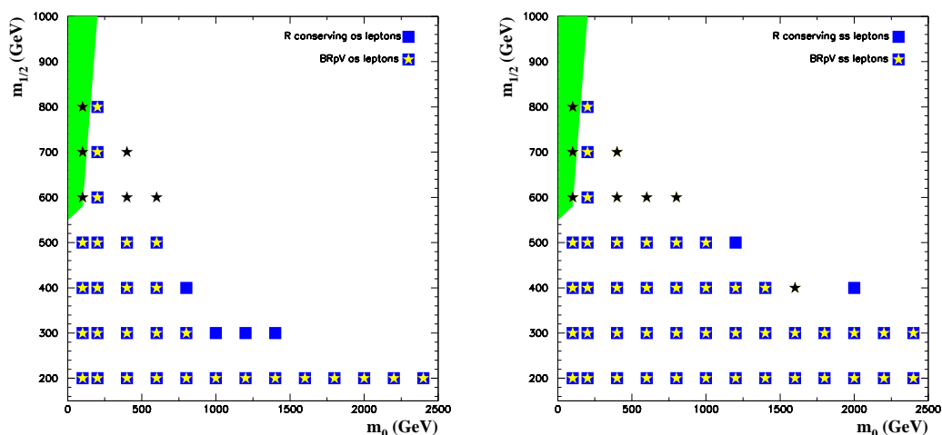
Figure 6: LHC discovery reach using opposite sign leptons (left panel) and same sign leptons (right panel) for the parameters used in figure 4.
