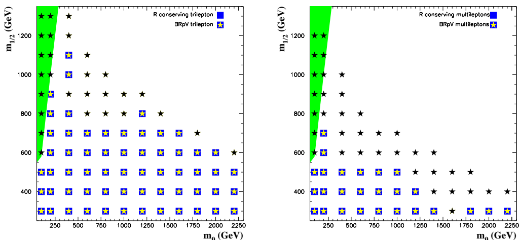
Figure 9: Same as figure 8 but for an integrated luminosity of 100 \text{ fb}^{-1} .
