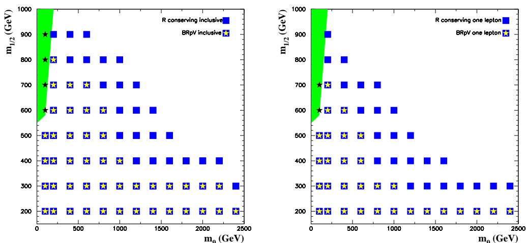
Figure 4: LHC discovery reach in the inclusive channel (left panel) and in the one lepton channel (right panel). We assumed \tan\beta = 10 , \mu > 0 , A_0 = -100 GeV, and an integrated luminosity of 10\text{ fb}^{-1} . The points leading to visible signal at the LHC are marked by a square for (R-parity-conserving) mSUGRA and by a star for the BRpV-mSUGRA case. The (green) shaded area indicates the region where the stau is the LSP. Points already excluded by LEP and Tevatron searches lie below the m_{1/2} values depicted in this figure.
