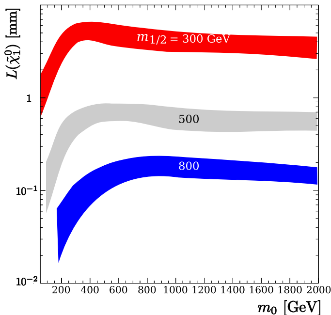
Figure 1: \tilde{\chi}_1^0 decay length versus m_0 for A_0 = -100 GeV, \tan\beta = 10 , \mu > 0 , and several values of m_{1/2} . The widths of the three shaded (colored) bands around m_{1/2} = 300, 500, 800 GeV correspond to the variation of the BRpV parameters in such a way that the neutrino masses and mixing angles fit the required values [40] within 3\sigma .
