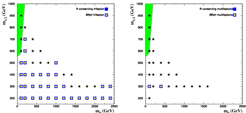
Figure 8: LHC discovery potential in the three lepton channel (left panel) and the multilepton one (right panel) for the parameters used in figure 4.
