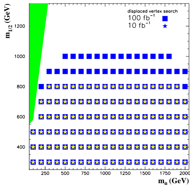
Figure 10: Discovery reach for displaced vertices channel in the m_0 \otimes m_{1/2} plane for \tan\beta = 10 , \mu > 0 , A_0 = -100 GeV. The stars (squares) stand for points where there are more than 5 displaced vertex signal events for an integrated luminosity of 10 (100) \text{fb}^{-1} . The marked grey (green) area on the left upper corner is the region where the stau is the LSP and the displaced vertex signal disappears. Points already excluded by LEP and Tevatron searches are below the m_{1/2} values depicted in this figure.
