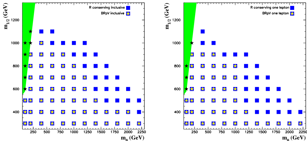
Figure 5: Same as figure 4 but for an integrated luminosity of 100\text{ fb}^{-1} .
